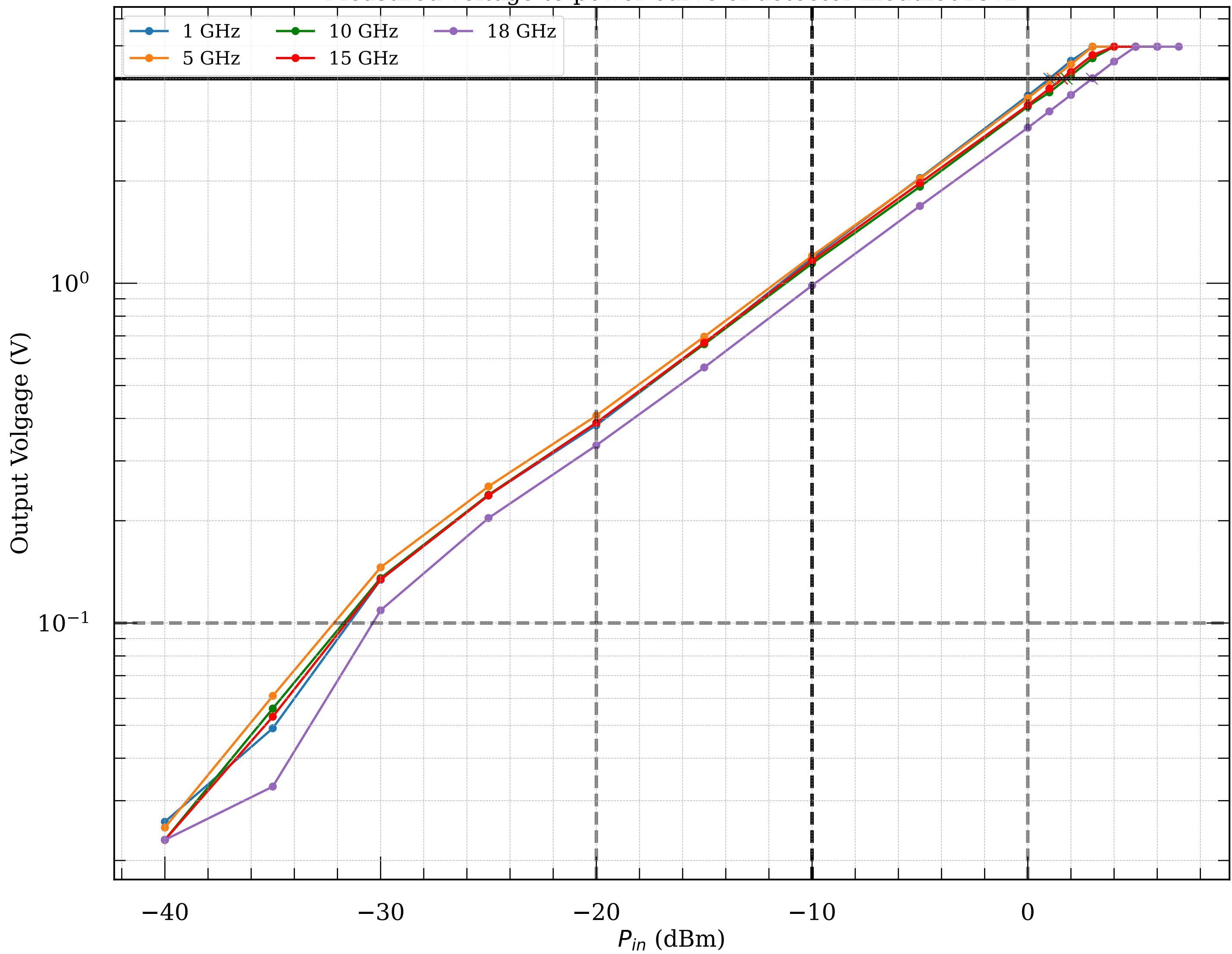
Measured voltage-to-power curve of detector module015v2
